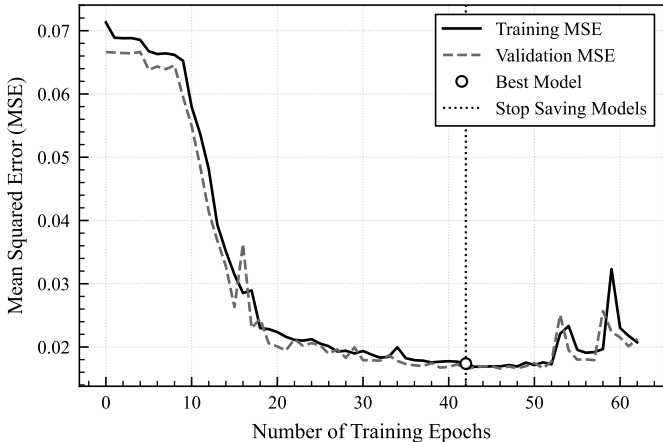
Learning Curve of LSTM Model for SolarPlant-2 (Gyeongju)
